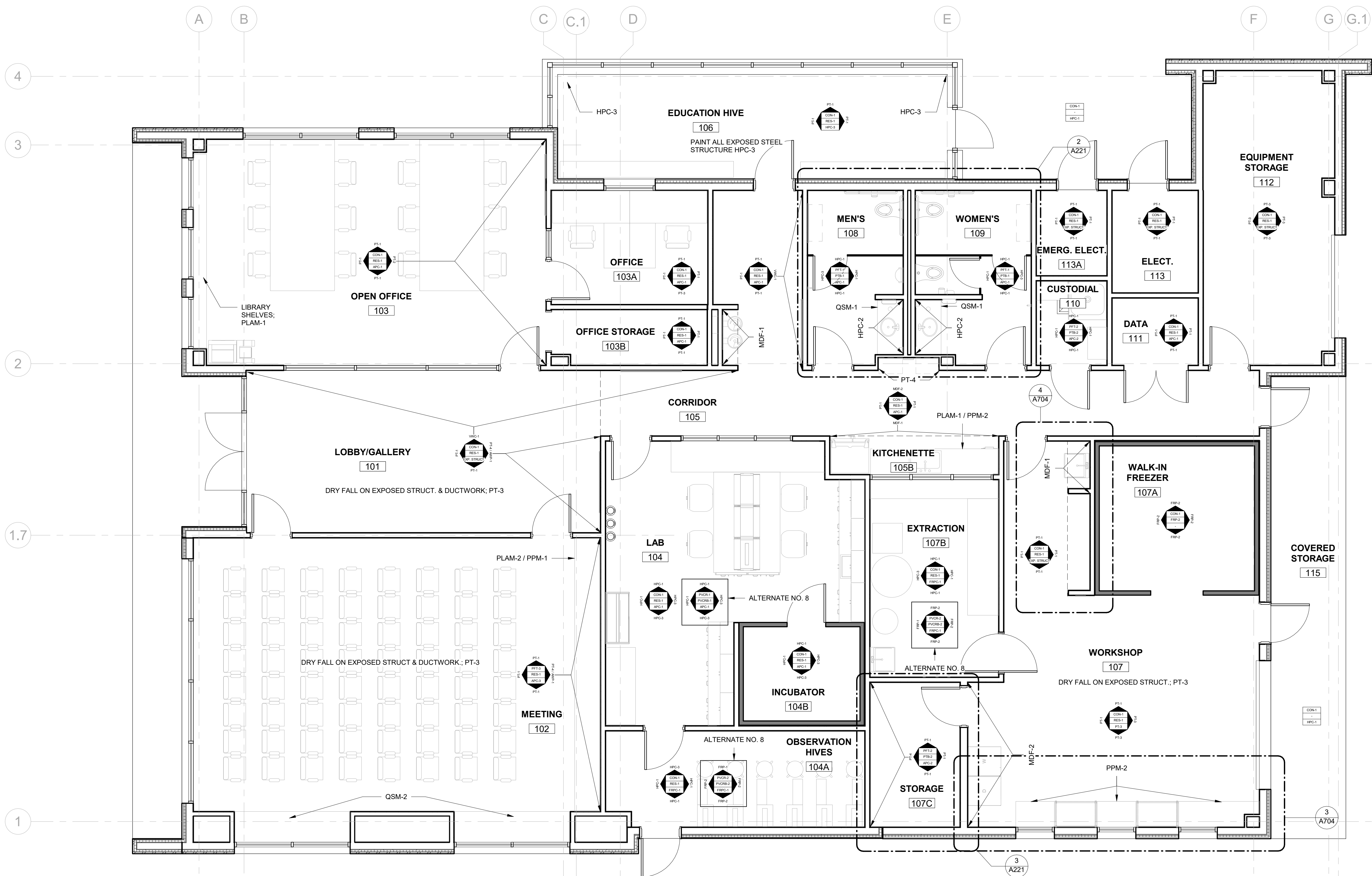
1 FINISH PLAN - ALTERNATE NO. 1 1/4" = 1'-0"
