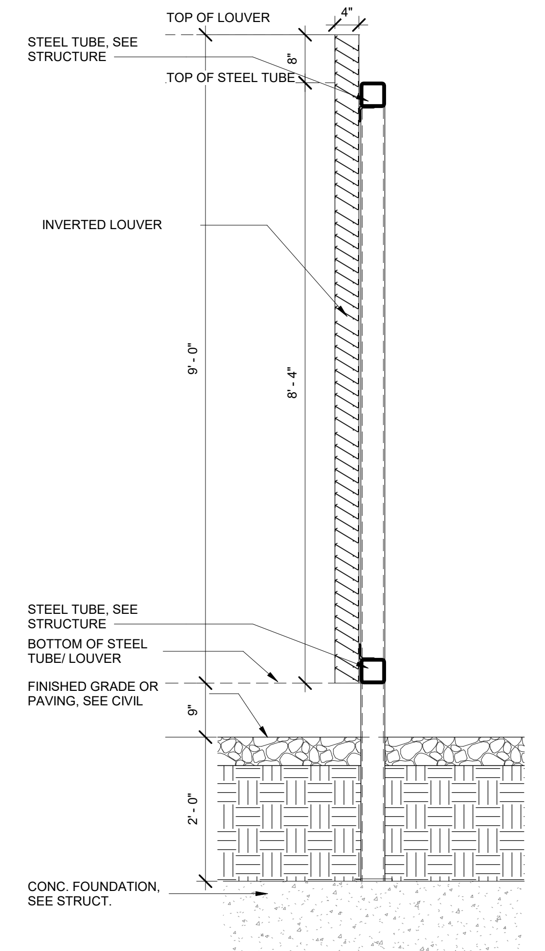
6 LOUVER DETAIL (ALTERNATE NO. 9) A112 3/4" = 1'-0"
