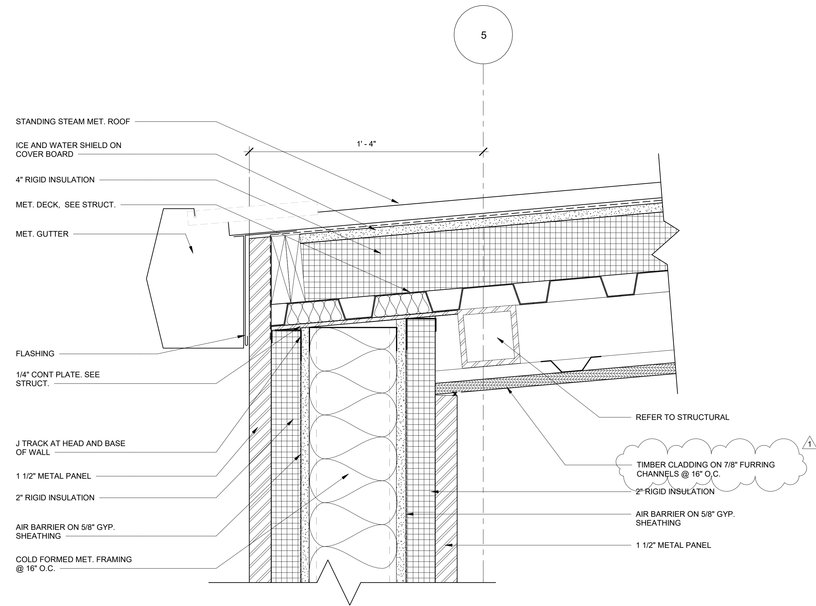
3 ROOF DETAIL A503 3" = 1'-0"
