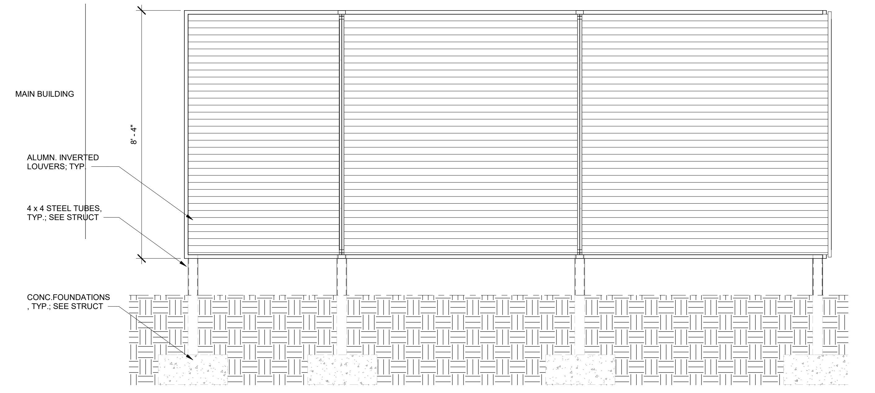
2 ELEVATION A112 1/2" = 1'-0"
