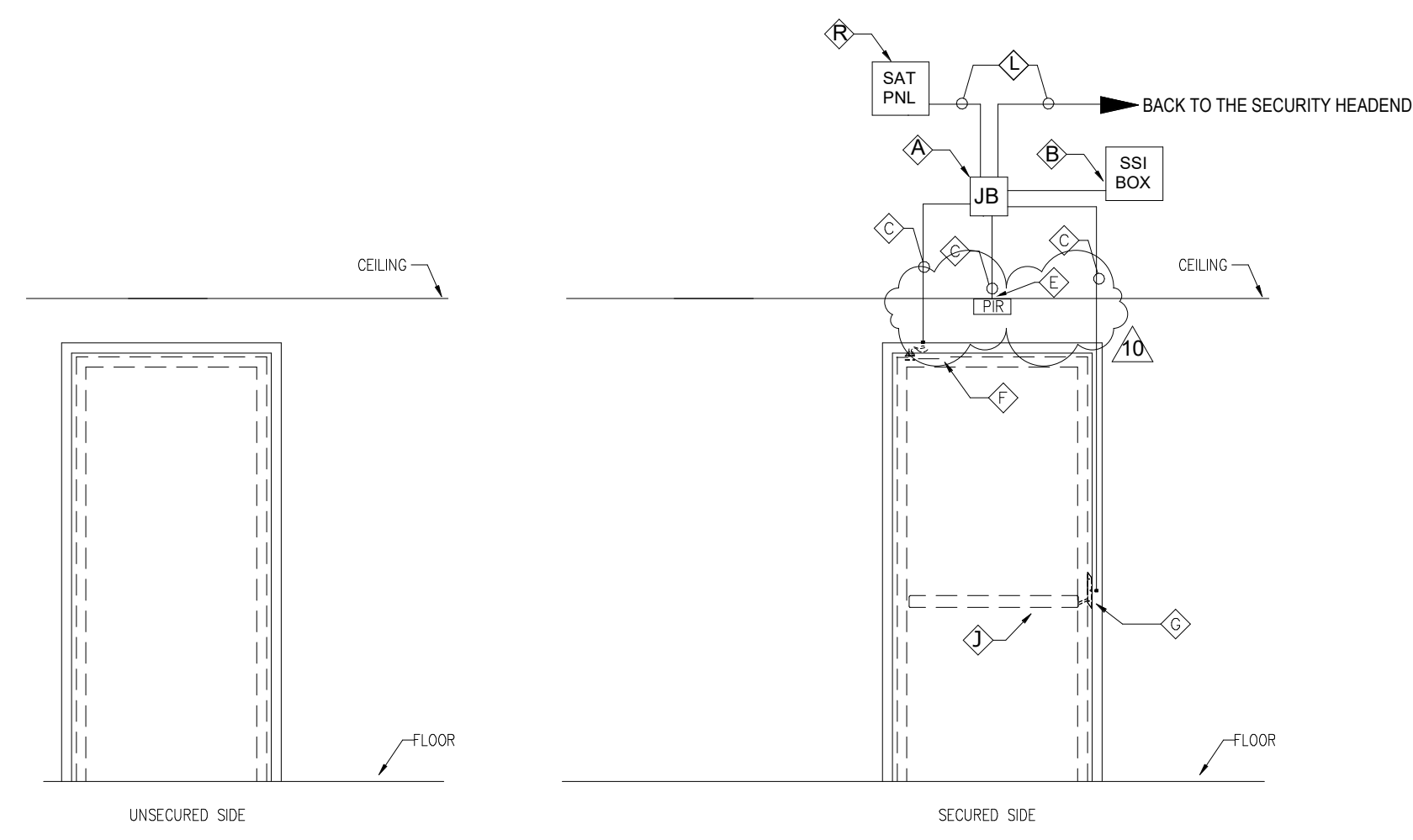
4 EXTERIOR SINGLE MP DOOR, MECHANICAL EXIT DETAIL Scale: N.T.S.
