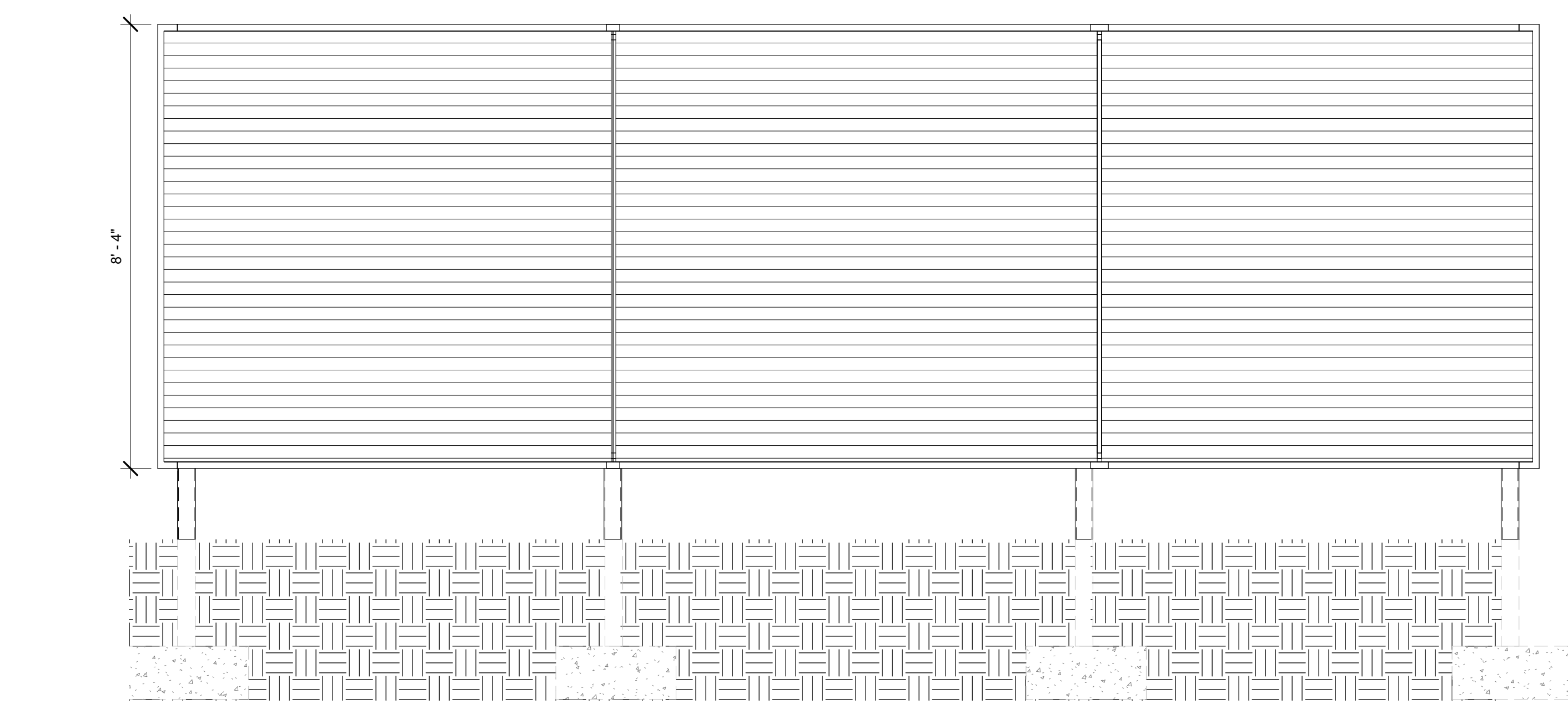
3 ELEVATION (ALTERNATE NO. 9) A112 1/2" = 1'-0"
